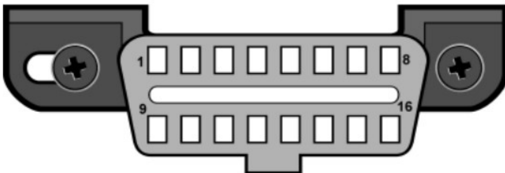
OBD II Diagnostic Link Connector
